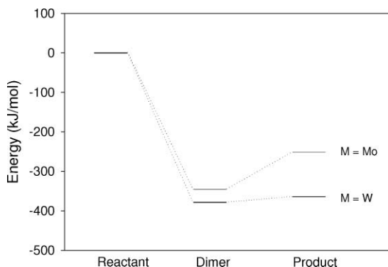
Fig. 1 Relative energies of reactant, intermediate and products for the reaction [\text{H}_2\text{N}]_3\text{M} + \text{CN}^- + \text{M}[\text{NH}_2]_3 \rightarrow [\text{H}_2\text{N}]_3\text{M}-\text{CN}-\text{M}[\text{NH}_2]_3^- \rightarrow [\text{H}_2\text{N}]_3\text{M}-\text{C}^- + \text{N}-\text{M}[\text{NH}_2]_3 ( \text{M} = \text{Mo}, \text{W} ) within the constraints of C_{3v} symmetry.
