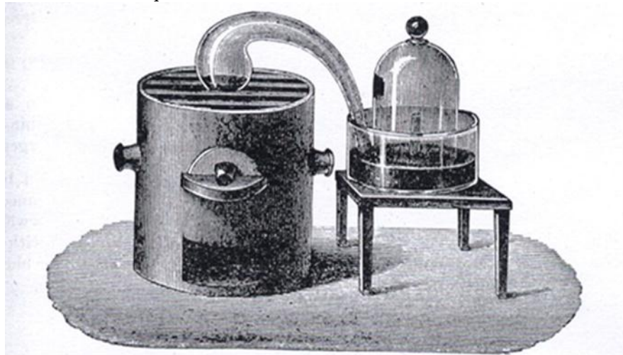
Fig. 2 Lavoisier's apparatus for studying the composition of air
