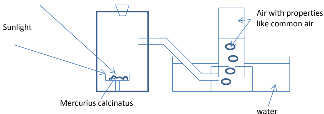
Fig.1 Heating of mercurius calcinatus to produce dephlogisticated air (oxygen) over water
