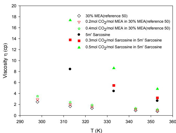
Figure 9. Viscosities of 5m' sarcosinate based solutions and 30% monoethanolamine (MEA) at temperatures of 298–353 K.
