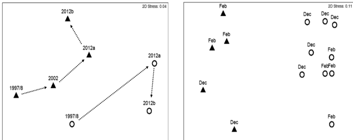
Figure 3: Assemblages associated with littoral sweeps in Lake Cootapatamba (▲) and Lake Albina (○) comparing: [a, left] previous overall assemblages (i.e. 1997/98 and 2002) with those in the present study and [b, right] site assemblages in both lakes on the two sampling occasions in 2012. In Fig. 3a, the February and December surveys in 2012 are represented as 2012a and 2012b, respectively, and arrows show progression through time.
