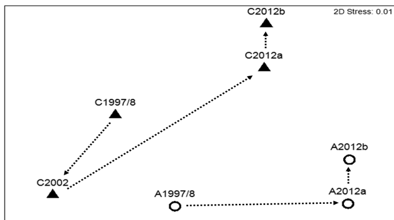
Figure 2: Assemblages associated with littoral cobbles in Lake Cootapatamba (▲) and Lake Albina (○) comparing: [a, left] previous overall assemblages (i.e. 1997/98 and 2002) with those in the present study and [b, below] site assemblages in both lakes on the two sampling occasions in 2012. In Fig. 2a, the February and December surveys in 2012 are represented as 2012a and 2012b, respectively, and arrows show progression through time.
