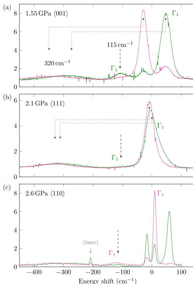
Figure 6. Uniaxial stress spectra including vibrational features. The upper trace (a) gives the spectra for \langle 001 \rangle stress and the central trace (b) for \langle 111 \rangle stress. In these cases the sample temperature was 150 K. (c) For \langle 110 \rangle stress the sample temperature was 10 K and the higher resolution was obtained by detecting emission from a small volume using masking. In all cases the feature at 115 \text{ cm}^{-1} is induced by the stress. It has the same polarization as the \Gamma_1 component of the ZPL ( \pi in the upper two traces and \sigma in lowest trace—see table 1). The first vibrational sideband at 320 \text{ cm}^{-1} can be seen to have the same polarization as the ZPL indicating the vibration has A_1 symmetry.
